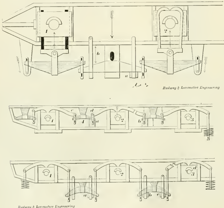
EXAMPLES OF UNDERHUNG SPRINGS.
